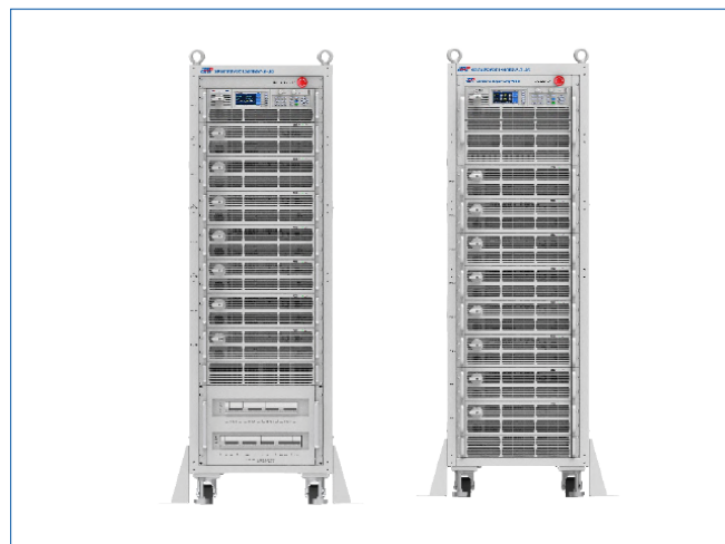
④ 560.0x1590.0x920.0 mm & 535kg
