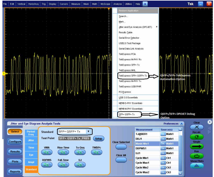
Tektronix SFP+ QSFPP+ Tx is developed on a Real Time Oscilloscope platform, which is the platform of choice for engineers designing their products around SFF-8431 & SFF-8634 technology. Option SFP-TX and SFP-WDP enable both an Automation Solution (for Compliance) and DPOJET Option (for Debug). Users can save up to 80% on testing time compared to manual testing. TWDPC - Transmitter Waveform Distortion Penalty for Copper Measurements are available with Option SFP-WDP. SFF-8431 SFP+ TWDPC based MATLAB code is integrated into the SFP-WDP option to make sure Engineers can use this measurement in the automated setup.
