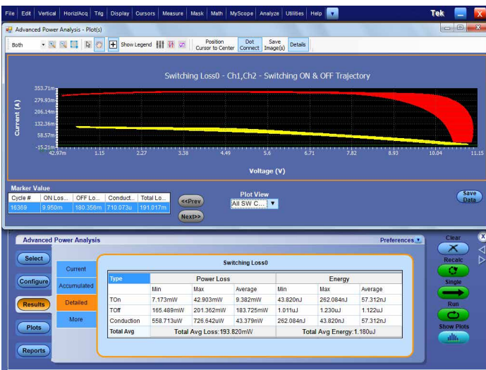
Power Measurement and Analysis Software (Option PWR) – DPOWR, Advanced Power Measurement and Analysis software allows the user to configure multiple measurements with custom defined settings, measure and analyze power dissipation in switching devices, and magnetic parameters in a single acquisition. The Trajectory plot computes turn-on loss, turn-off loss and Conduction loss parameters for each cycle. Measurements such as Phase, Conduction loss, amplitude, and Voltage harmonics provide more insight to Input/Output characterization of power supplies. A single mht format file with append feature provides an easy way of generating reports which include measurements, test results, and plot images.
