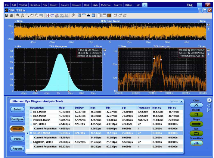
DPOJET Jitter and Eye Diagram Analysis – Simplify identifying signal integrity concerns, jitter, and their related sources with DPOJET software. DPOJET provides the highest sensitivity and accuracy available for real-time oscilloscopes.
