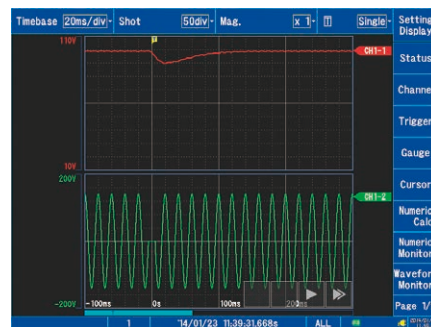
• Example of recording the instantaneous waveform and RMS level waveform during a momentary outage of an AC power supply (using the MR8905)
