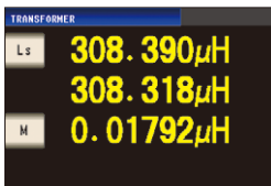
Transformer measurement mode Mutual inductance measurement screen
