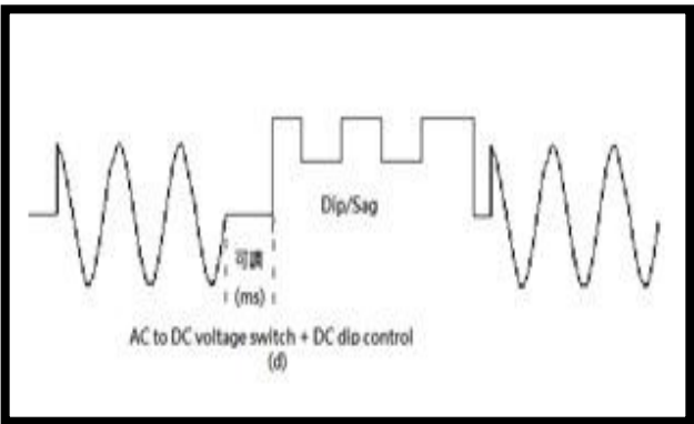
Voltage waveform test requirement
