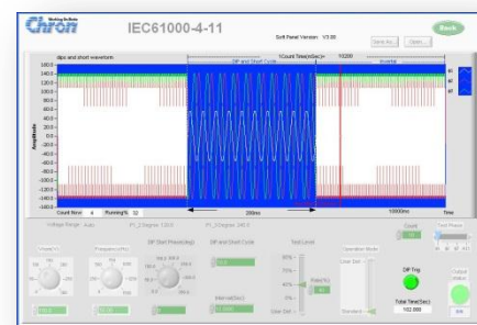
Voltage DIP, Short Interruption, Variation Regulation Test
