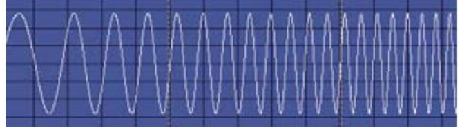
Output voltage waveform based on frequency of slew rate setting
