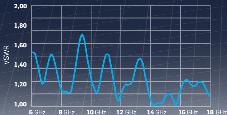
DR-01 - VSWR
