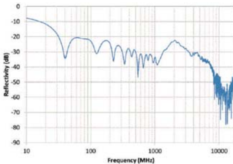
DSH-1250H DuraSorb™ Polystyrene Hybrid Absorber Typical Reflectivity
