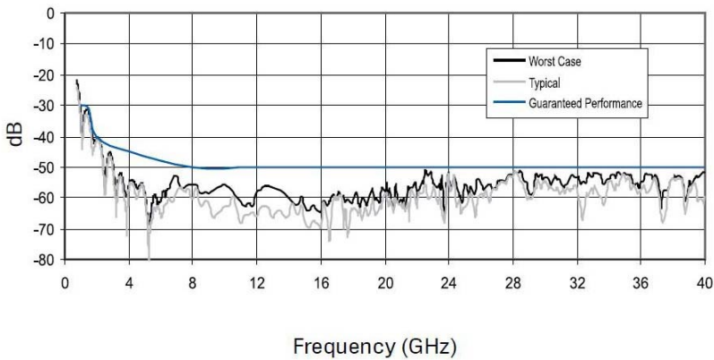
EHP-8PCL Measured Reflections at Normal Incidence
