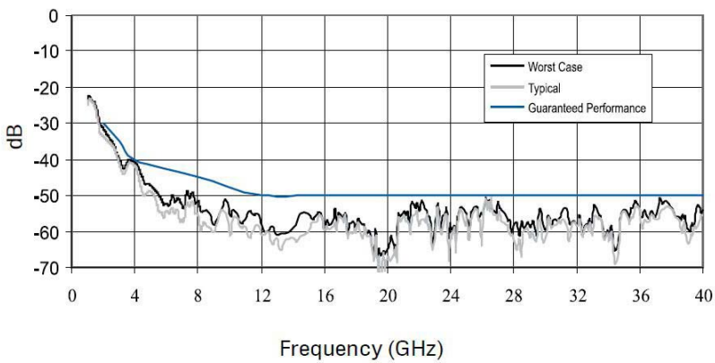
EHP-5PCL Measured Reflections at Normal Incidence
