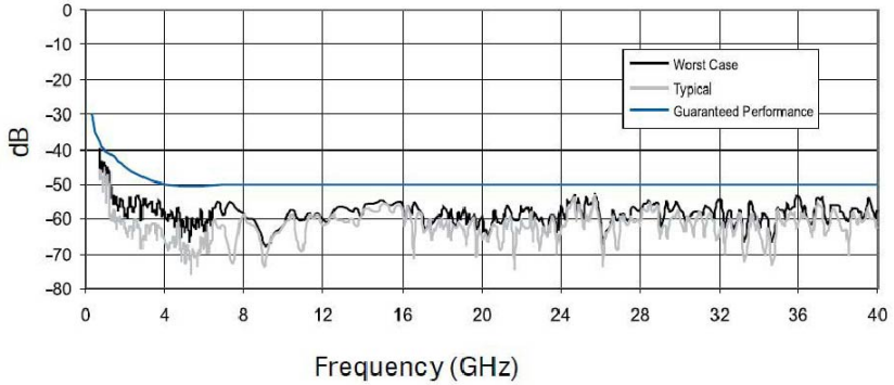
EHP-24PCL Measured Reflections at Normal Incidence
