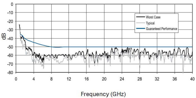
EHP-12PCL Measured Reflections at Normal Incidence
