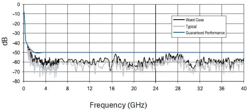
EHP-36PCL Measured Reflections at Normal Incidence
