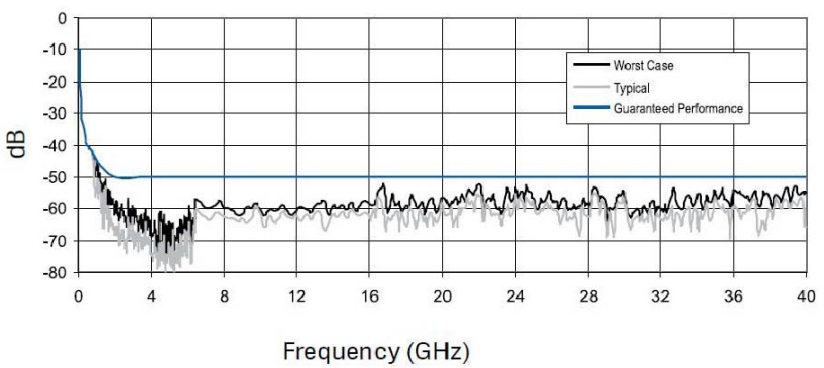
EHP-48PCL Measured Reflections at Normal Incidence
