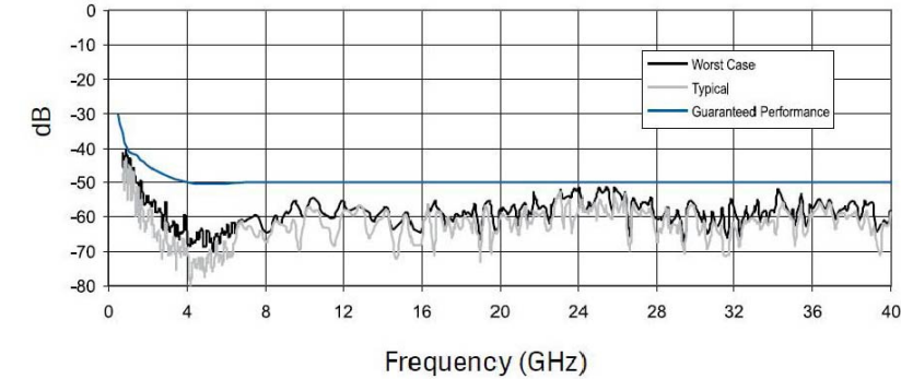
EHP-18PCL Measured Reflections at Normal Incidence
