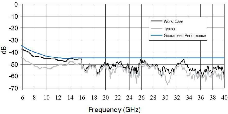
EHP-3PCL Measured Reflections at Normal Incidence
