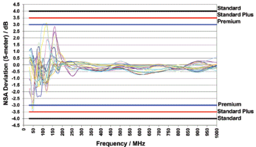
Measured NSA Deviation (5-meter), 30 MHz to 1 GHz
