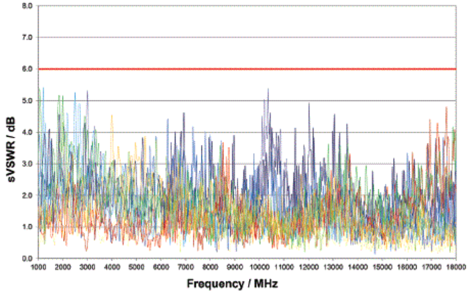
Measured sVSWR Deviation (3-meter), 1 GHz to 18 GHz
