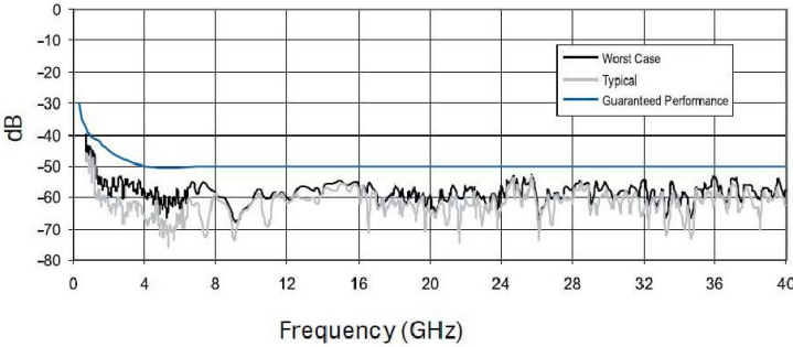
EHP-24PCL Measured Reflections at Normal Incidence
