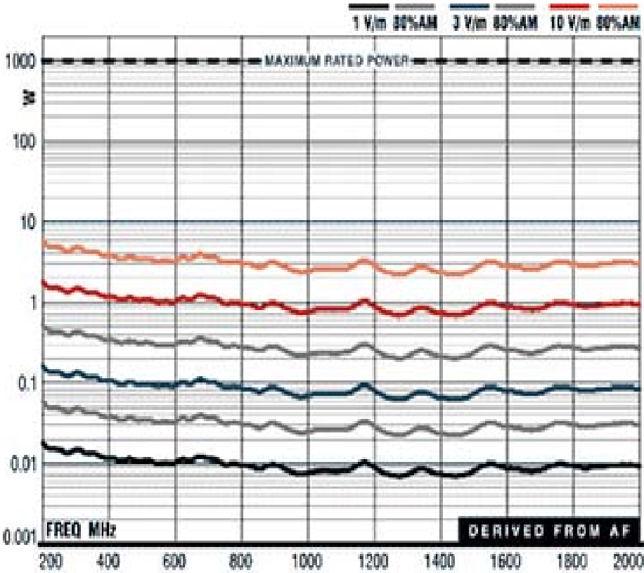
3148B Log Periodic Dipole Array Antenna Forward Power at 1 m
