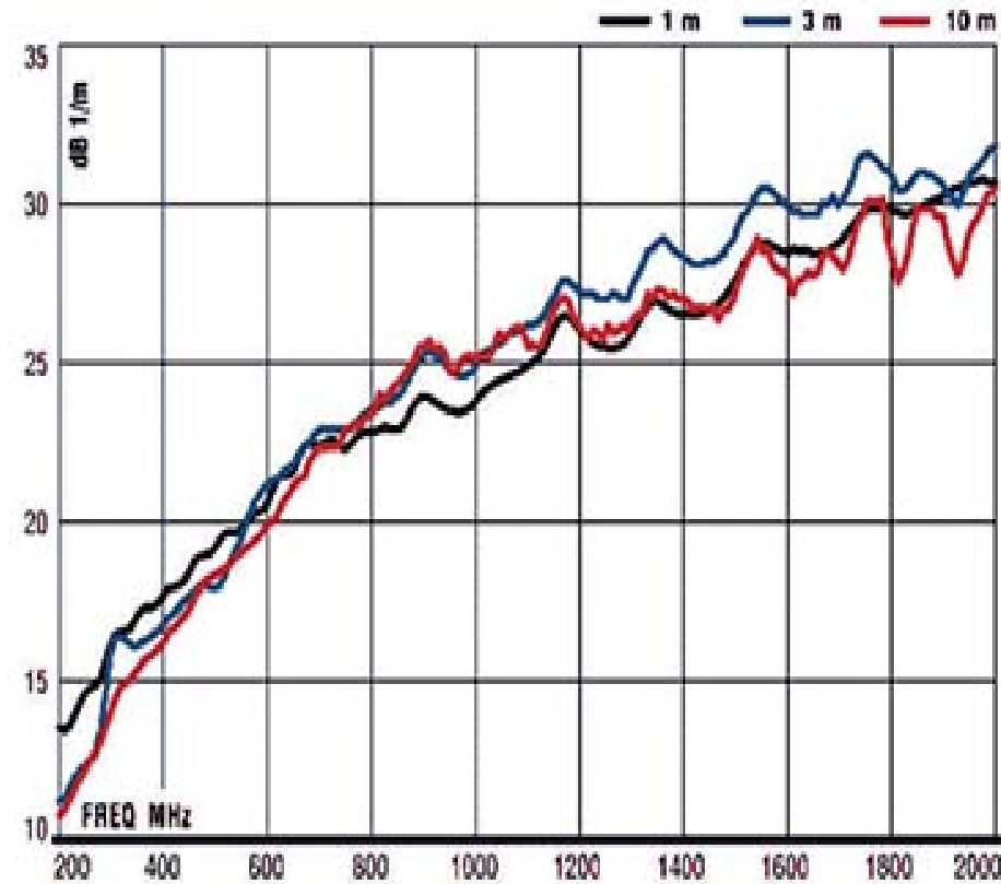
3148B Log Periodic Dipole Array Antenna Factor
