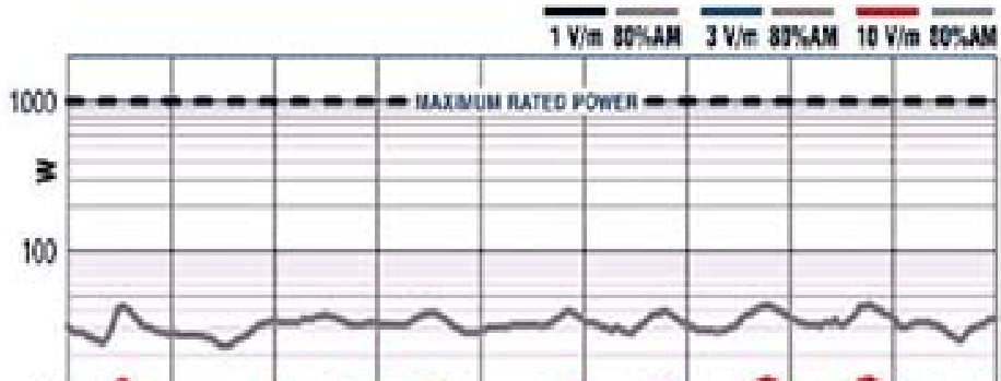
3148B Log Periodic Dipole Array Antenna Forward Power at 3 m
