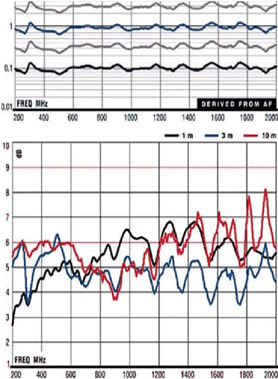
3148B Log Periodic Dipole Array Antenna Gain
