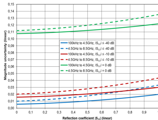
Typical accuracy of reflection magnitude and reflection phase measurements for the R&S®ZND Analysis conditions: S_{21} = 0 , cal. power –10 dBm, meas. power –10 dBm, Base unit or K1 installed.
