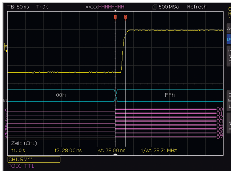
8 bit DAC signal change
