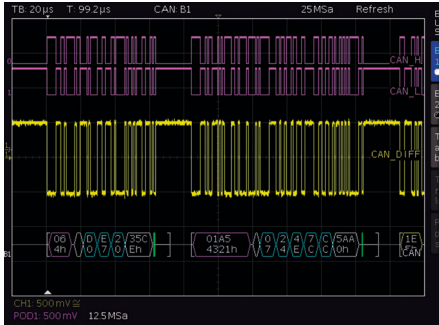
HEX decoded CAN bus signal
