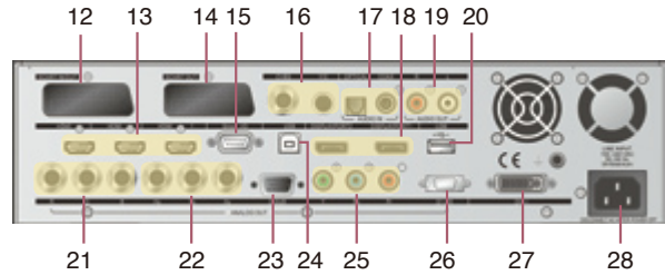
Rear View
